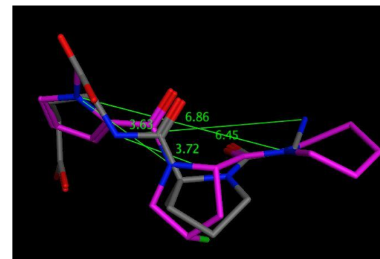
Computer modeling (Shape similarity / topological similarity). Purple – compounds from the sub-library
