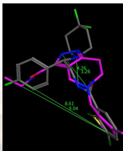
Computer modeling (Shape similarity / topological similarity). Purple – compounds from the sub-library
