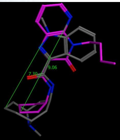
Computer modeling (Shape similarity / topological similarity). Purple – compounds from the sub-library
