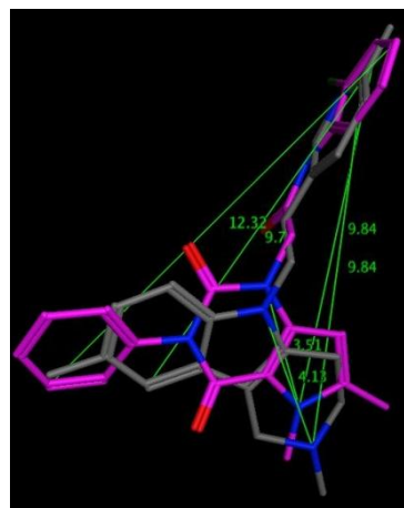
Computer modeling (Shape similarity / topological similarity). Purple – compounds from the sub-library
